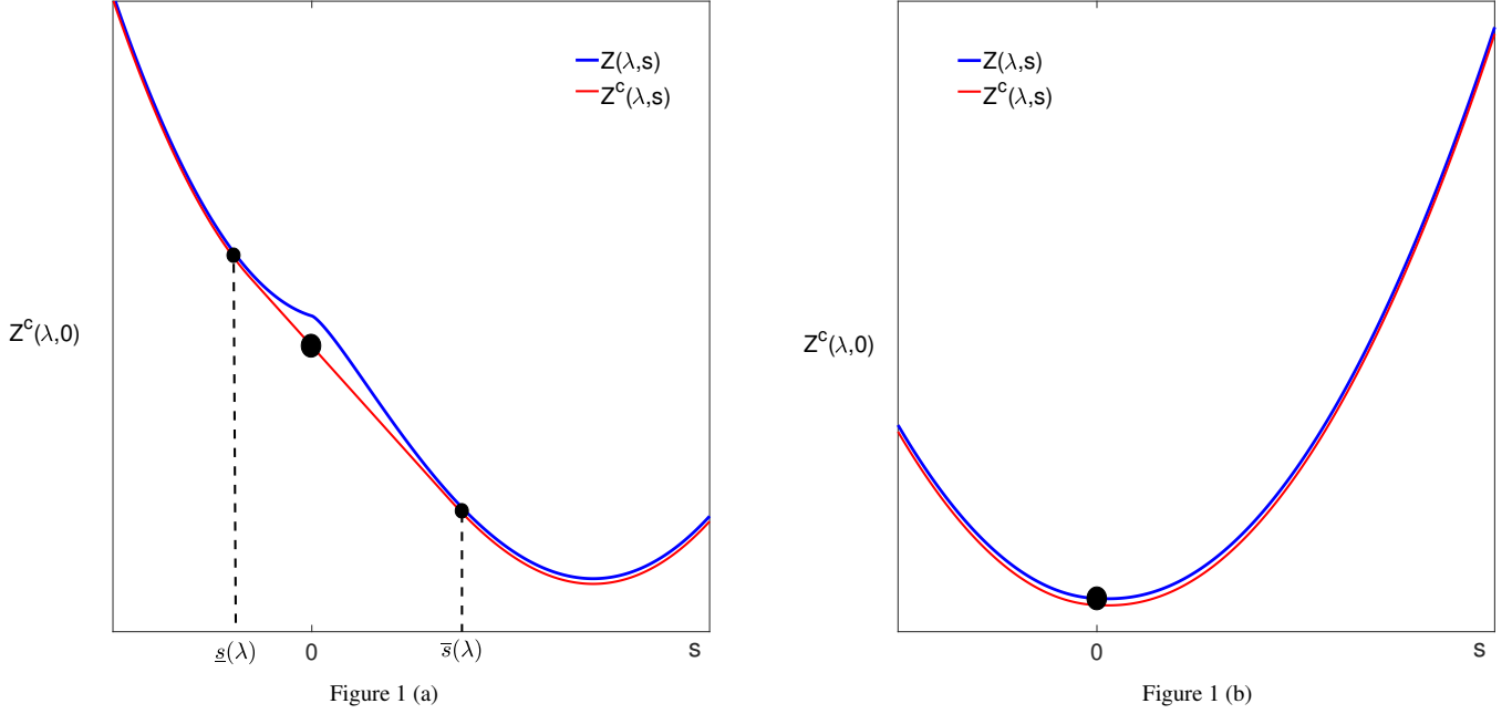
Figure 1: Illustration of the Principal's best response.
